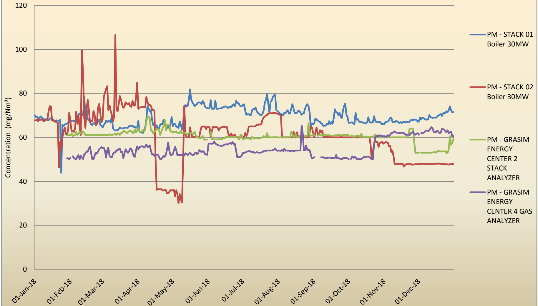
Annual Emission Trend of Particulate Matter in M/s. Grasim Industries Ltd., Dist. Ujjain (M.P.)
