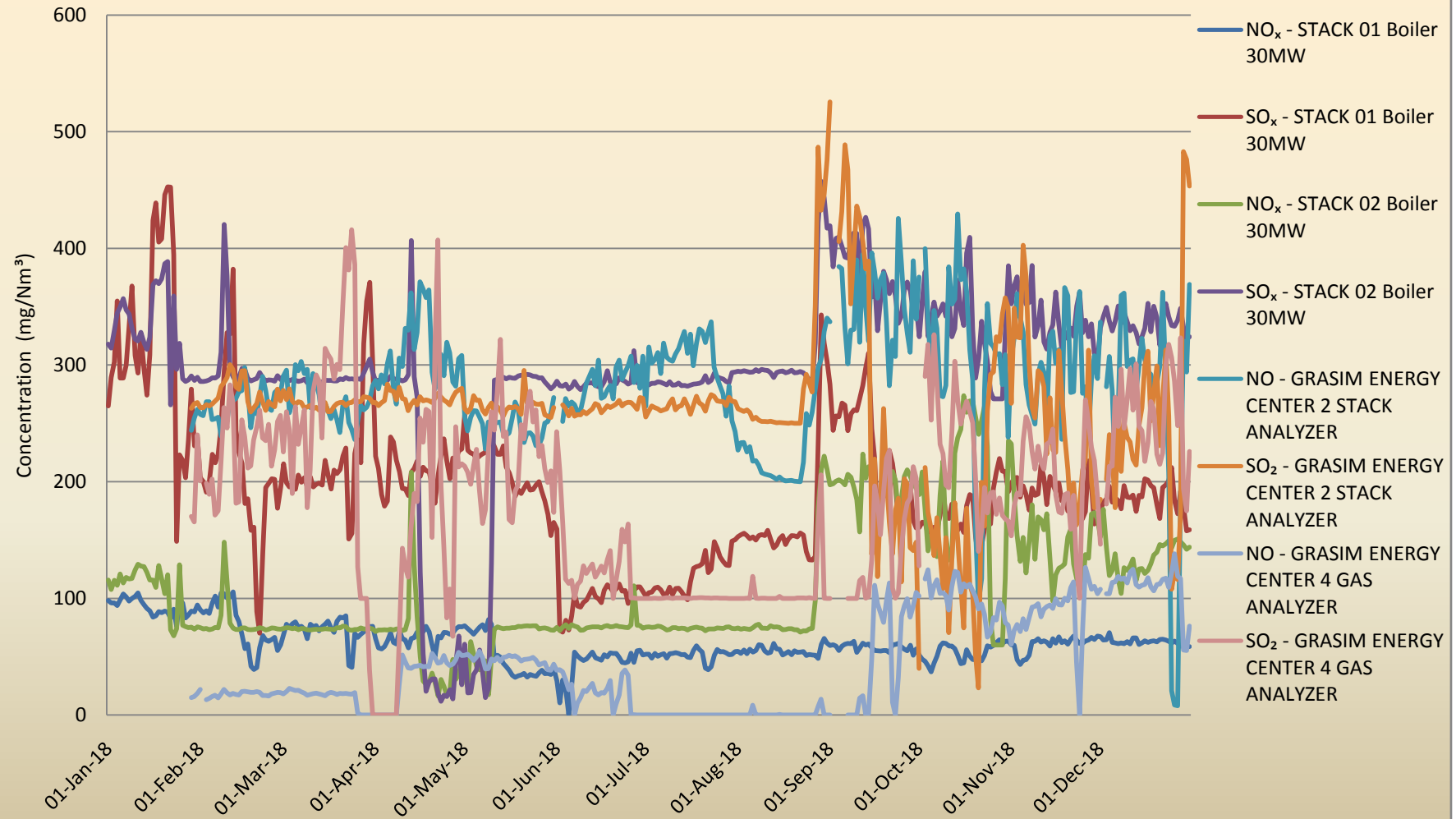
Annual Emission Trend of Gaseous in M/s. Grasim Industries Ltd., Dist. Ujjain (M.P.)
